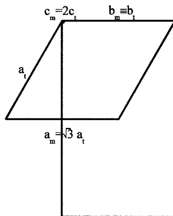
Fig. 3. Drawing of the I2 structure of \text{CaSO}_4 \cdot 0.5\text{H}_2\text{O} projected parallel to [001] . Inset: metrical relationships existing between the unit cell of the trigonal P3_121 substructure and that of the I2 monoclinic structure.
