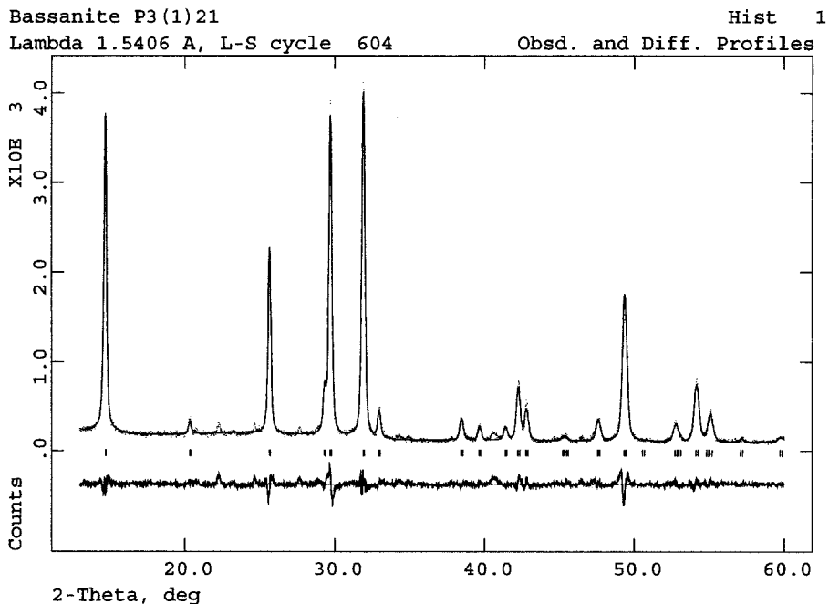
Fig. 2. b) Experimental (dots) and calculated (continuous line) plots for the P3 21 structure of \text{CaSO}_4 \cdot 0.5\text{H}_2\text{O} .
