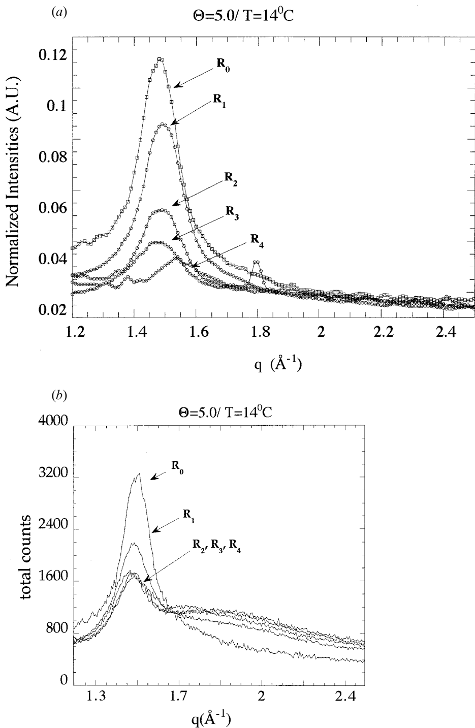
Figure 27. The effect of the interaction of the two DHPs on the diffraction peak due to the DMPC bilayer's acyl-chain distances (all spectra have been acquired for 1000 s). (a) Nifedipine at different molar ratios of DHP to DMPC: R_0 = 0 ; R_1 = 4 \times 10^{-4} ; R_2 = 4 \times 10^{-3} ; R_3 = 6 \times 10^{-3} ; R_4 = 5 \times 10^{-1} . The spectra are normalized at the DMPC
