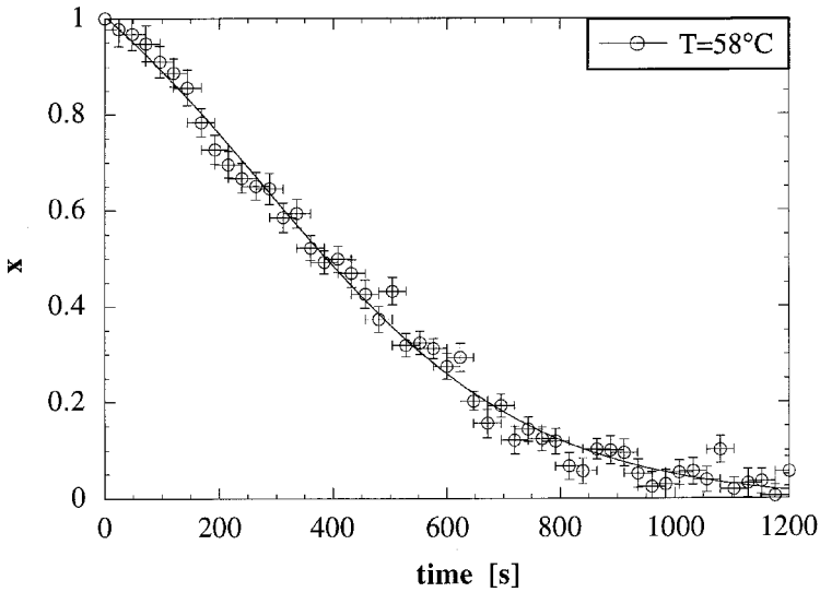
Figure 12. Plot of x against t at T = 58^\circ\text{C} during melting, together with its sigmoidal fit. The horizontal error bars represent the acquisition time; the vertical error bars are the standard deviation of the x distribution. (Reprinted with permission from [12]; copyright 1997 by Marcel Dekker, Inc.)
