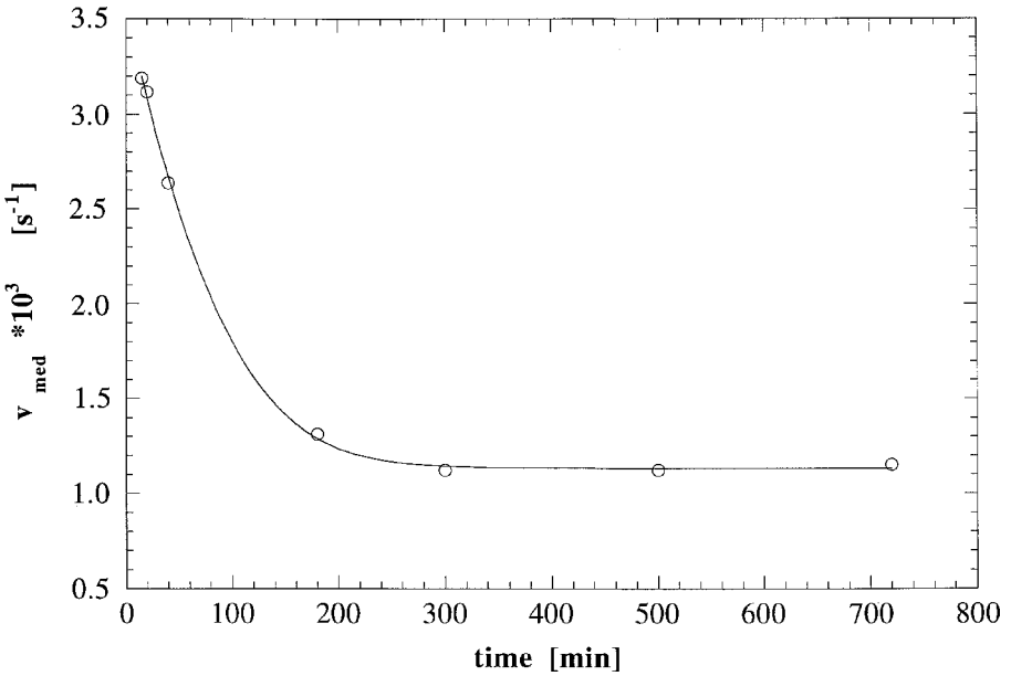
Figure 22. Plot of the crystallization rate obtained from the curves showed in figure 21, fitted by the theoretical Liquori-Tripiciano model T = T(1) = 112 \text{ }^\circ\text{C} . (Reprinted with permission from [38]; copyright 1999 by Marcel Dekker, Inc.)
