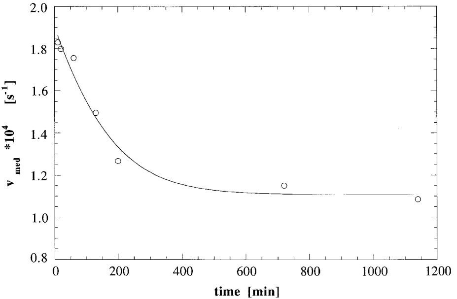
Figure 23. The same plot as in figure 22 for the temperature T = T(2) = 116 \text{ }^\circ\text{C} . (Reprinted with permission from [38]; copyright 1999 by Marcel Dekker, Inc.)
