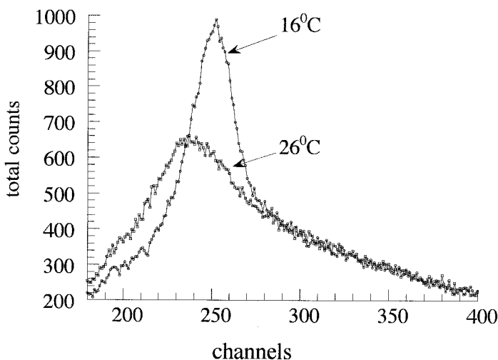
Figure 28. DMPC diffraction spectra at two different temperatures before and after the PT. The main peak corresponds to the quasicrystalline PB' phase; the lower peak corresponds to the liquid-like (amorphous) L\alpha phase. (Reprinted with permission from [39]; copyright 1998 by Elsevier Science B.V.)
