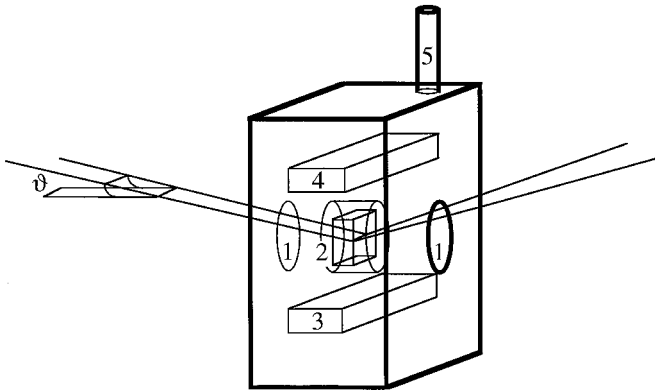
Figure 8. Schematic design of the variable-temperature cell: 1, Mylar windows; 2, sample holder; 3, heat source (electric heater); 4, cold source (frozen liquids or liquid-nitrogen container); 5, vacuum pipe. (Reprinted with permission from [37]; copyright 1997 by Marcel Dekker, Inc.)
