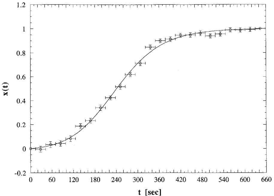
Figure 11. Plot of the transformation coordinate x(t) , where the abscissa and ordinate error bars are analogous to those of figure 10: (—), the Liquori-Tripiciano law fit. \tau_1 = 3921.8 \pm 495.1 s and \tau_2 = 85.6 \pm 3.4 s are its phenomenological parameter values. (Reprinted with permission from [11]; copyright 1996 by Marcel Dekker, Inc.)
